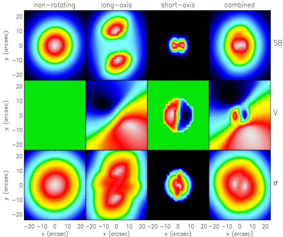
Figure 1. Kinematics of a triaxial Abel model. From top to bottom: the surface brightness (SB), the mean velocity ( V ) and velocity dispersion ( \sigma ). From left to right: non-rotating, (outer and inner) long-axis and short-axis rotating components, and a (luminosity weighted) combination. The non-rotating components have zero mean velocity. The short-axis component is limited due to the finite extent of Abel models. The kinematically decoupled core in the combined model is a typical signature of triaxiality observed in e.g. NGC4365 (Davies et al. 2001).
